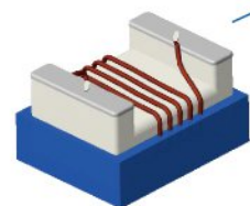
片式陶瓷绕线电感, 用于ADAS, POC, NFC 等 Wire wound chip ceramic inductor, used on ADAS, POC, NFC, etc
